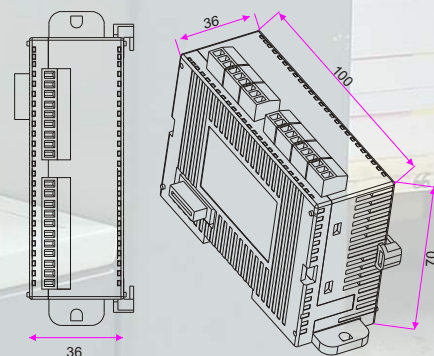
Fig. B FlexiLogics® expansion module
