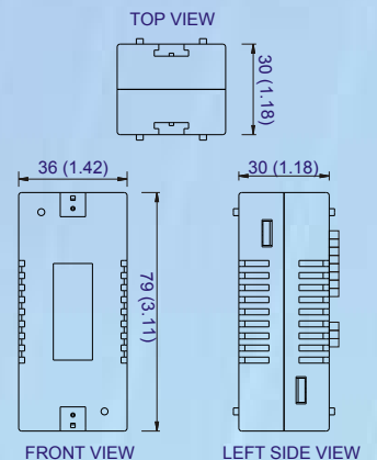
Expansion Modules
